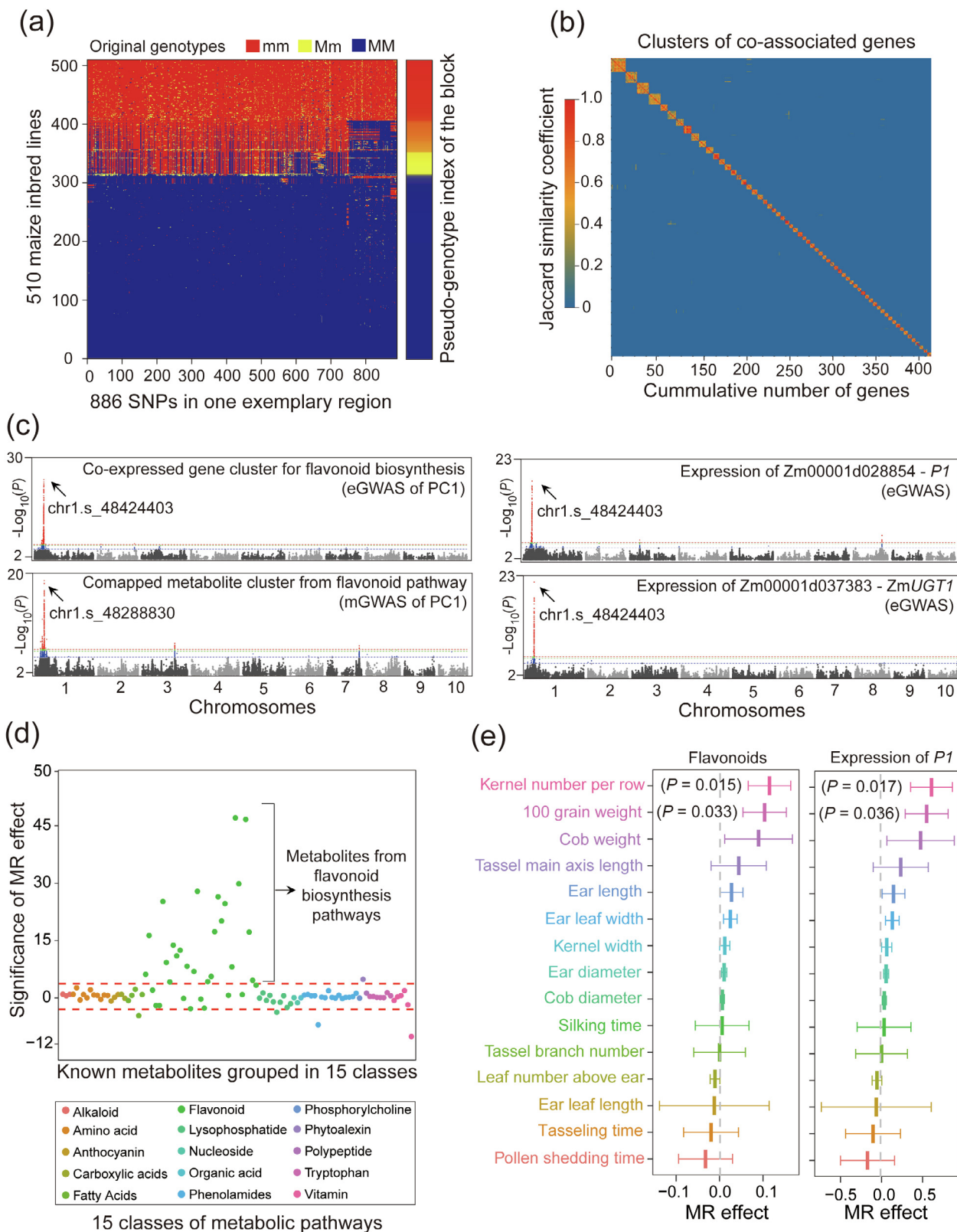
Fig. 1. Four major analytical modules of MODAS. (a) Module of dimensionality reduction. The pseudo-genotype index reflects the overall genotypic variation of an exemplary region (Chr1: 142.0 to143.5 Mb). “M” and “m” represent the major and minor alleles of the 886 SNPs, respectively. (b) Module of regional association (RA) analysis. The heatmap illustrates the 62 clusters of co-associated genes identified by RA analysis. (c) Module of expression GWAS (eGWAS) and metabolome GWAS (mGWAS). P1 gene is located in the genomic region peaked at Chr1: s_48424403. ZmUGT1 gene is located at Chr6: 123,804,940 to 123,806,574, regulated by P1 in trans . (d) Module of Mendelian randomization (MR). Causal relations between the P1 gene and 135 known metabolites were inferred. The y axis is -\log_{10}(P) , in which the P represents the statistical significance of the MR effect estimated by \chi^2 test. The red dashed lines represent the significance threshold ( P = 1 \times 10^{-5} ) for positive and negative MR effects. (e) MR-based estimation of the contribution of flavonoid levels and P1 expression levels to the 15 agronomic traits of maize.
